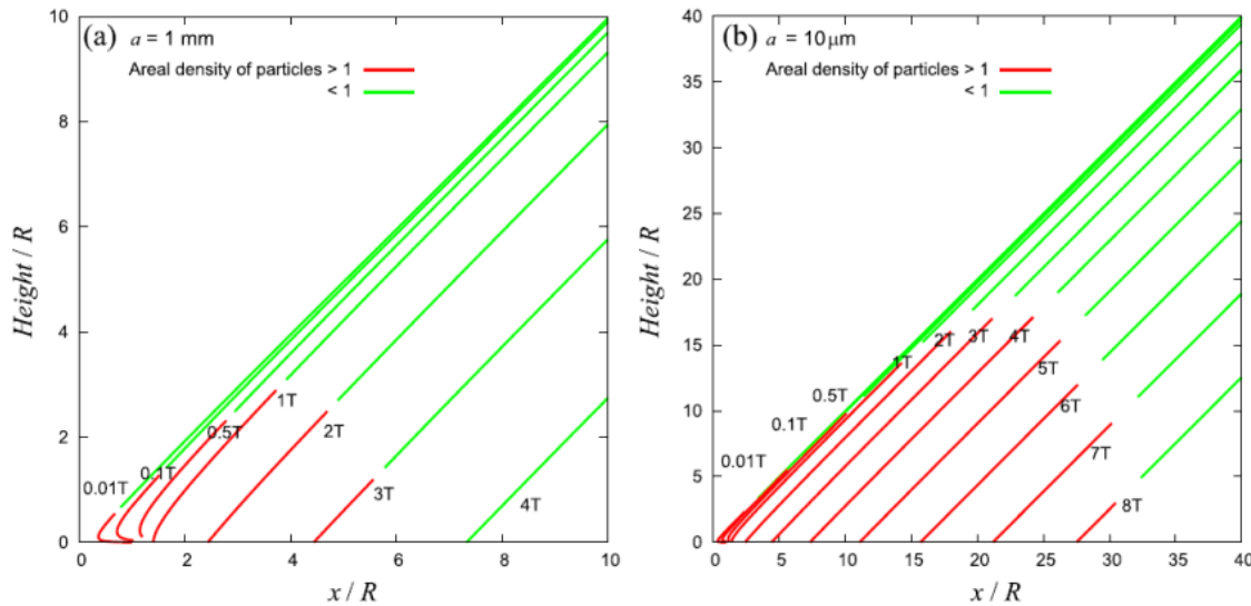
Fig. 6 The cross section of the ejecta curtain proceeding with time, assuming a typical sand target ( C_2 = 0.64 and \mu = 0.41 ), and the radius of constituent ejecta particles is (a) 1 mm and (b) 10 \mu\text{m} . The horizontal axis shows the distance x from the impact point and the vertical axis shows the height from the target surface, both being normalized by the final crater radius R . The time labeled for each curtain is normalized by the crater growth time T = 0.92(R/g)^{1/2} for a typical sand target, where g is the surface gravity (Holsapple and Housen 2007). With g and R being 2.6 \times 10^{-4} \text{ m/s}^2 and 5 m, respectively, T is calculated to be 128 sec. The red lines show a dense part of curtains with an areal density of particles > 1 , while the green lines show a sparse part
