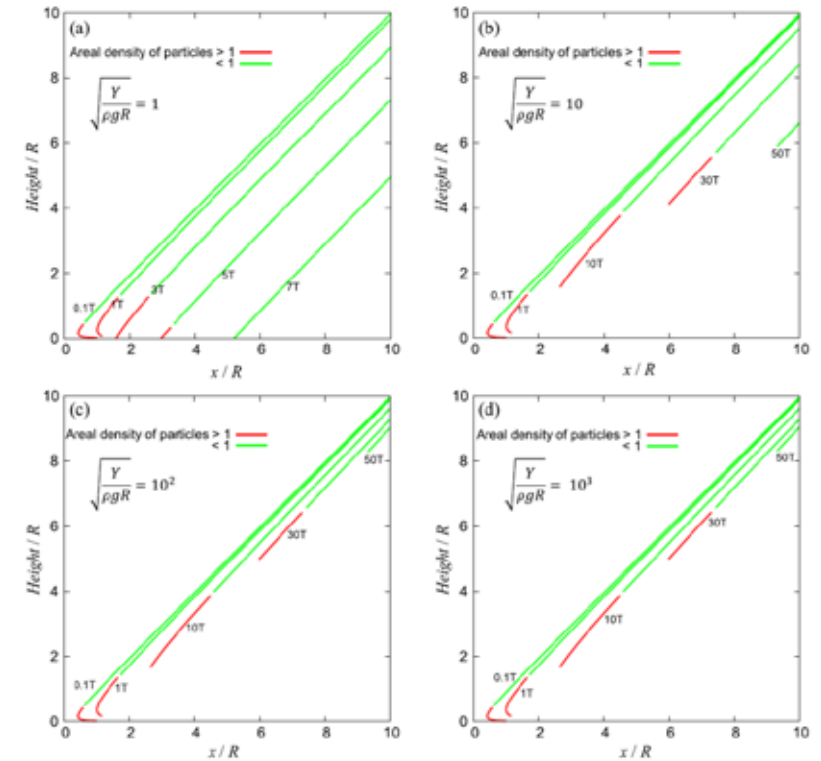
Fig. 11 Same as Fig. 6, but assuming the strength regime scaling law with parameters of C_3 = 0.53 and \mu = 0.55 (Holsapple and Holsapple 2011). The ejecta curtains proceed differently, depending on the target strength Y with (Y/\rho g R)^{1/2} = (a) 1, (b) 10, (c) 100, and (d) 1000. The crater growth time T is given by T = 0.44R/(Y/\rho)^{1/2} for a typical rock target (Holsapple and Housen 2007). Here we assume R = 1\text{m} , then (a) T = 27.3 sec, (b) 2.73 sec, (c) 0.273 sec, and (d) 0.0273 sec. When giving the areal density of curtains, we assume the radius of the constituent ejecta particles to be 1 mm
